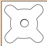
SF-1418-5 WALLER PLATE Sheet Thickness : 5mm Weight : 0.550 kg.
